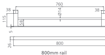
800mm rail
