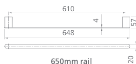
650mm rail
