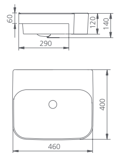
Semi-recessed basin No tap hole
