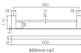
600mm rail
