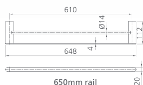
650mm rail
