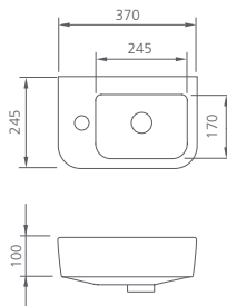
Compact wall hung basin
