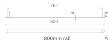
800mm rail
