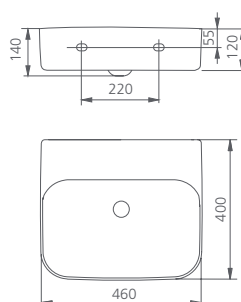
Wall hung basin No tap hole
