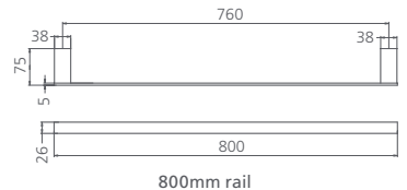
800mm rail
