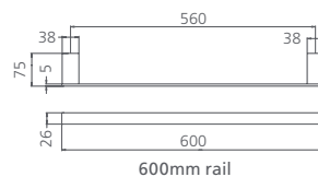
600mm rail
