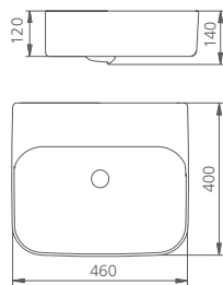
Counter top basin No tap hole
