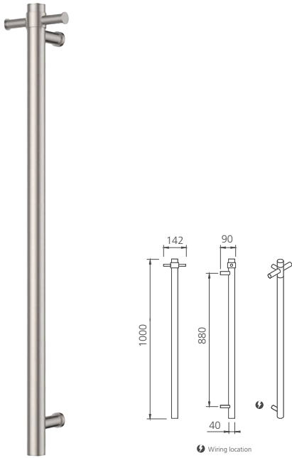
Venice heated vertical towel rail
