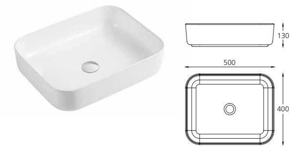
Counter top rectangular basin Bowl capacity 14.9L / NA3711
