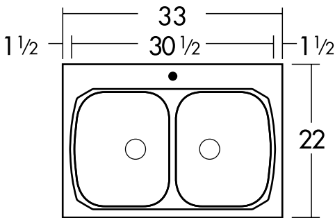
Maxi Basin 1 13 3 / 4 x 16 1 / 2 x 8" deep 6.2 Gallon Capacity
